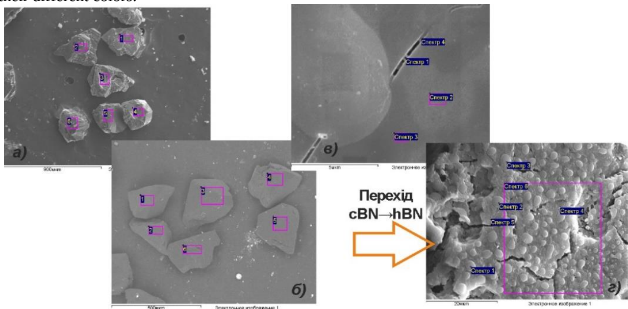
Fig. 1 – Analysis of the mechanism of laser radiation ( \lambda = 1.06 \mu\text{m} ) effect on CNB grains of KV 250/200 grade
